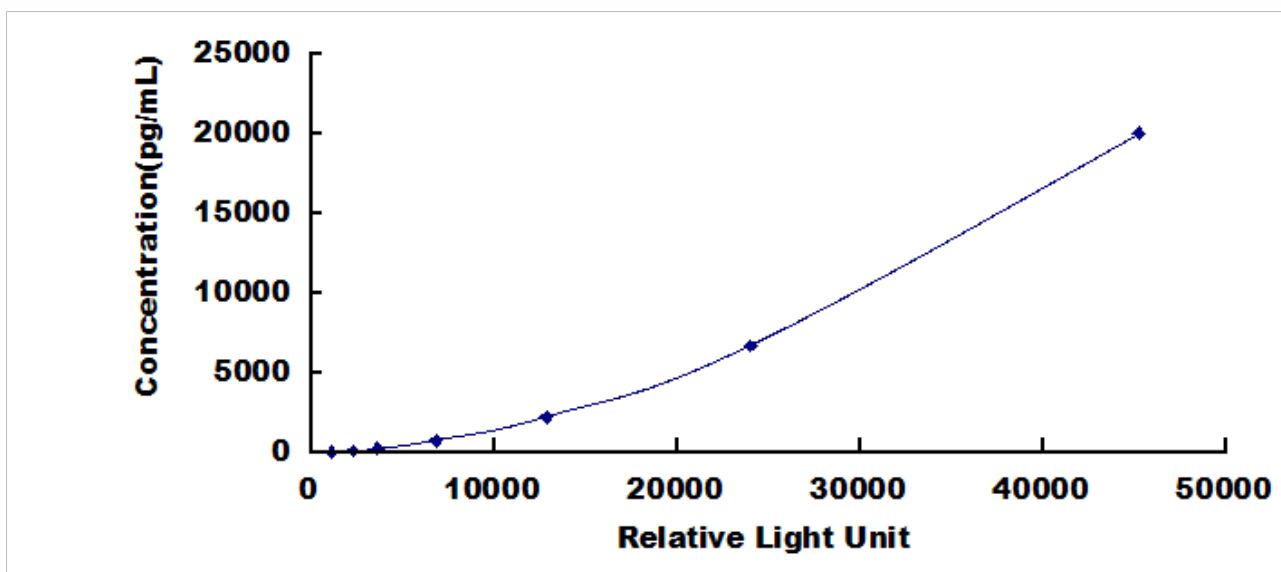
Typical Standard Curve for Growth Hormone, Rat CLIA.
