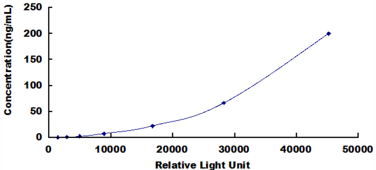
Typical Standard Curve for C4c, Human CLIA.
