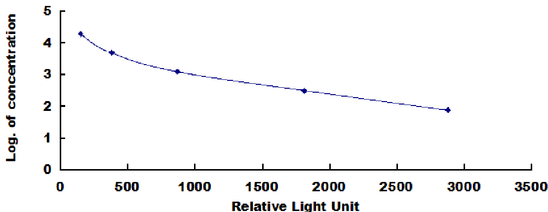
Typical Standard Curve for INS, Rat CLIA.
