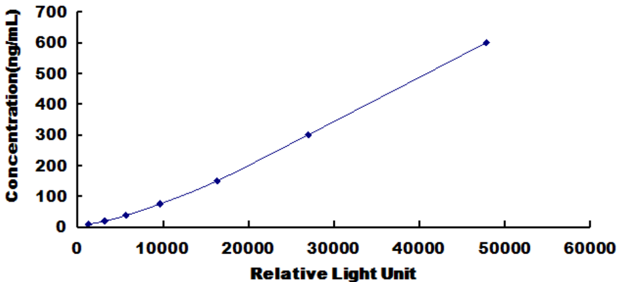
Typical Standard Curve for Human IGFBP7 CLIA.
