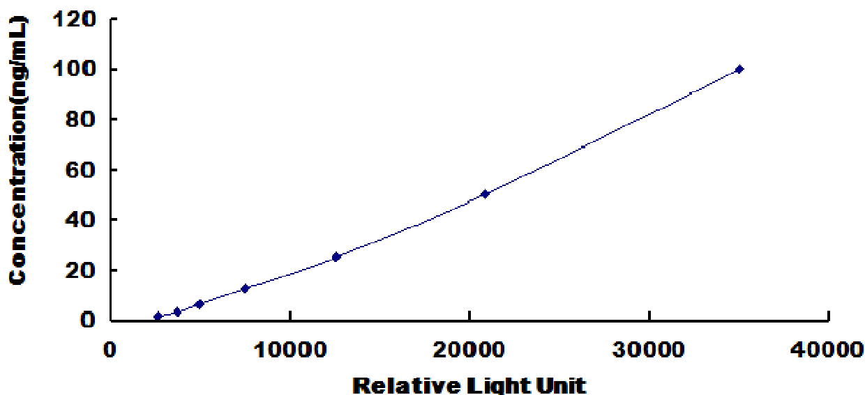
Typical Standard Curve for Human SULF2 CLIA.
