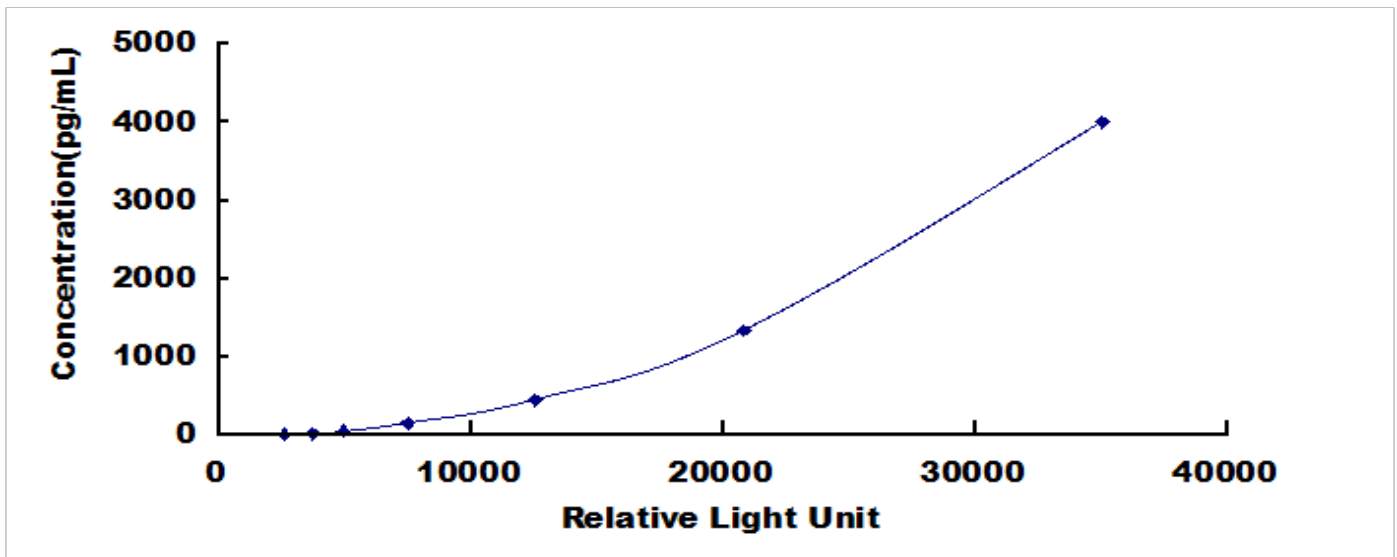
Typical Standard Curve for CLCF1, Human CLIA.
