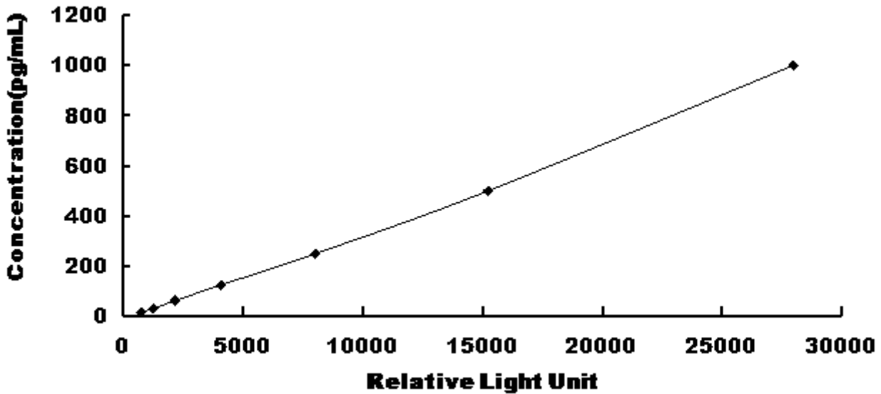
Typical Standard Curve for Gallus FGF4 CLIA.
