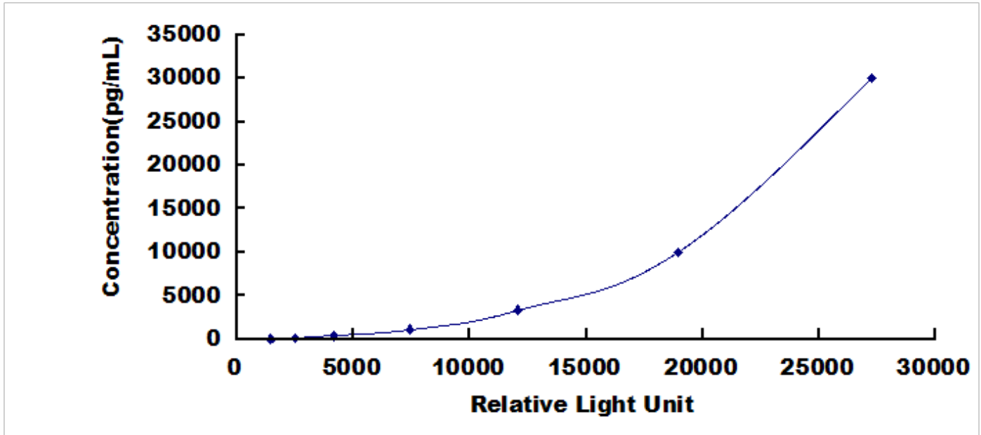
Typical Standard Curve for MMP1, Human CLIA.
