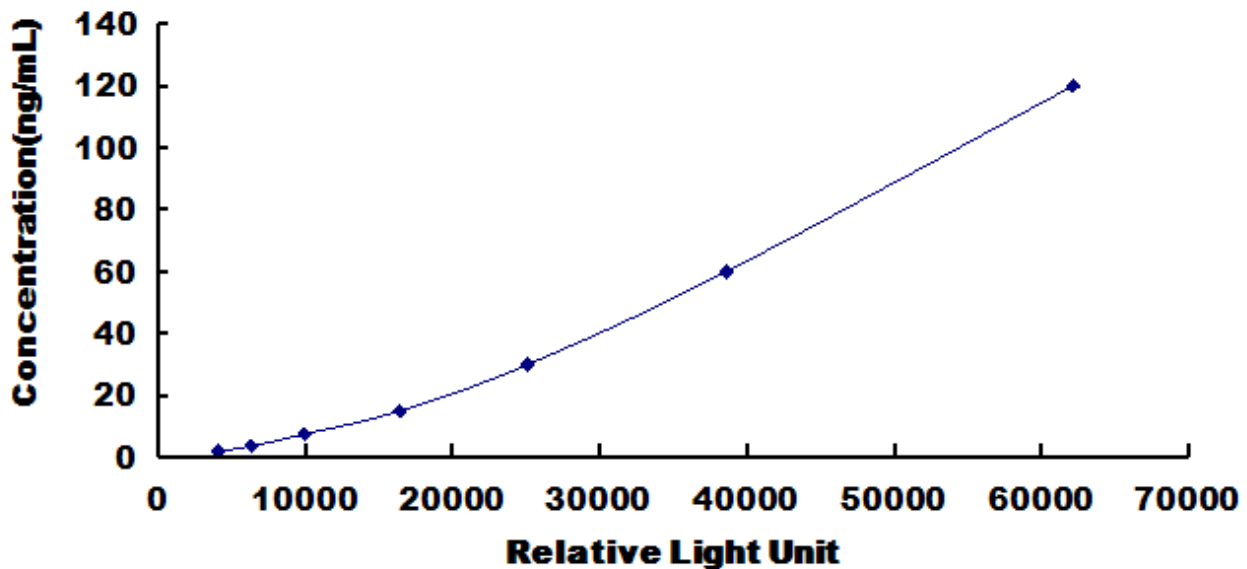
Typical Standard Curve for Human TFF3 CLIA.
