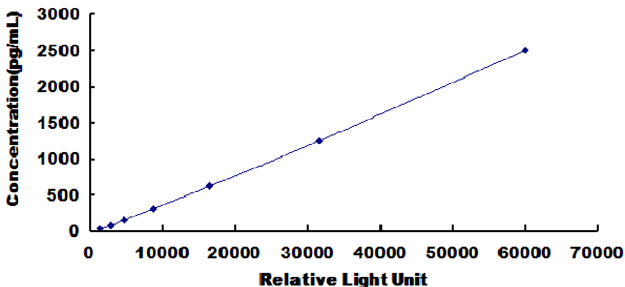
Typical Standard Curve for Human NT-ProBNP CLIA.
