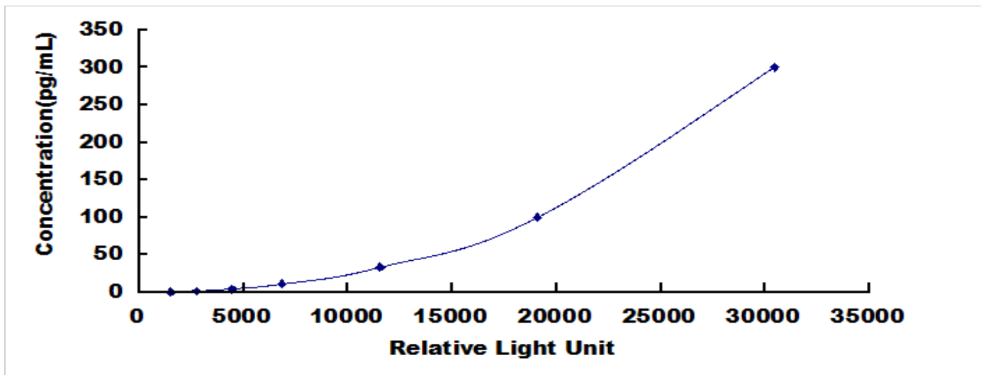
Typical Standard Curve for IL6, Rat CLIA.
