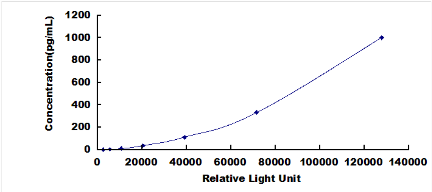
Typical Standard Curve for IFNg, Rat CLIA.
