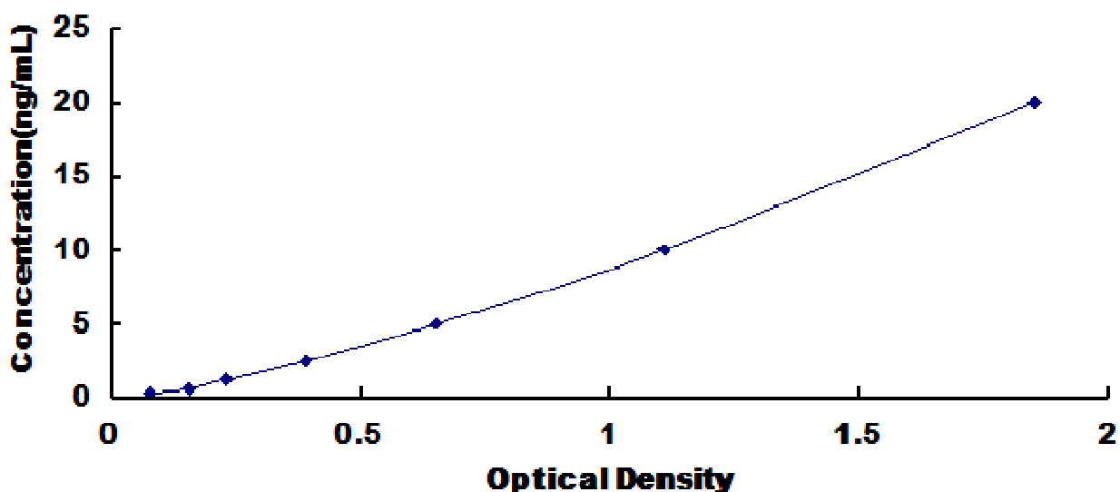
Typical Standard Curve for VCP, Rat ELISA.
