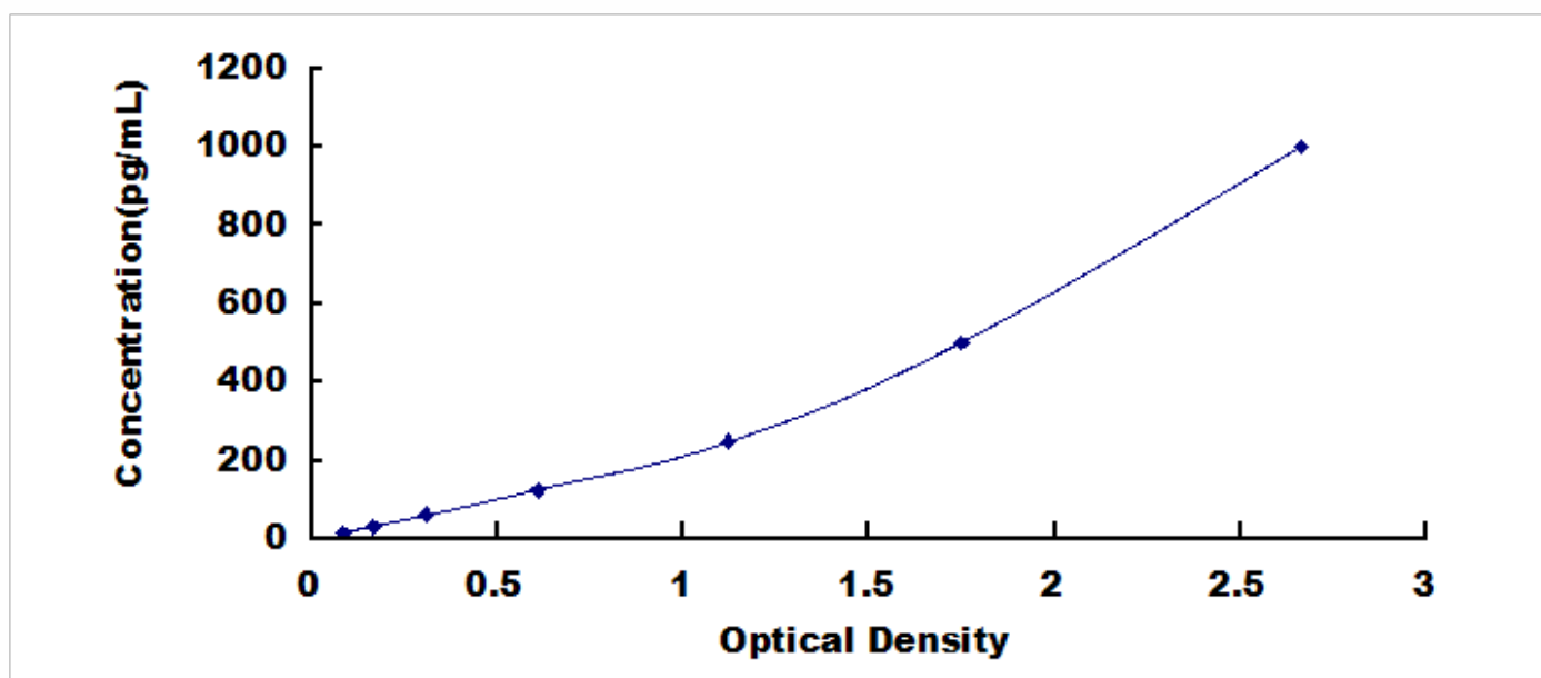
Typical Standard Curve for TNFSF4, Human ELISA.
