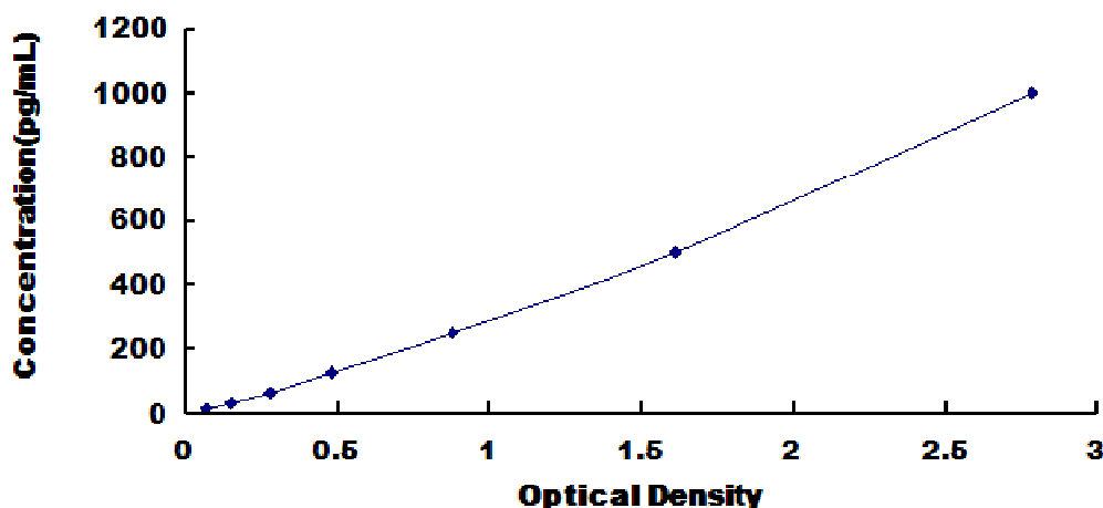
Typical Standard Curve for TGFb2, Bovine ELISA.
