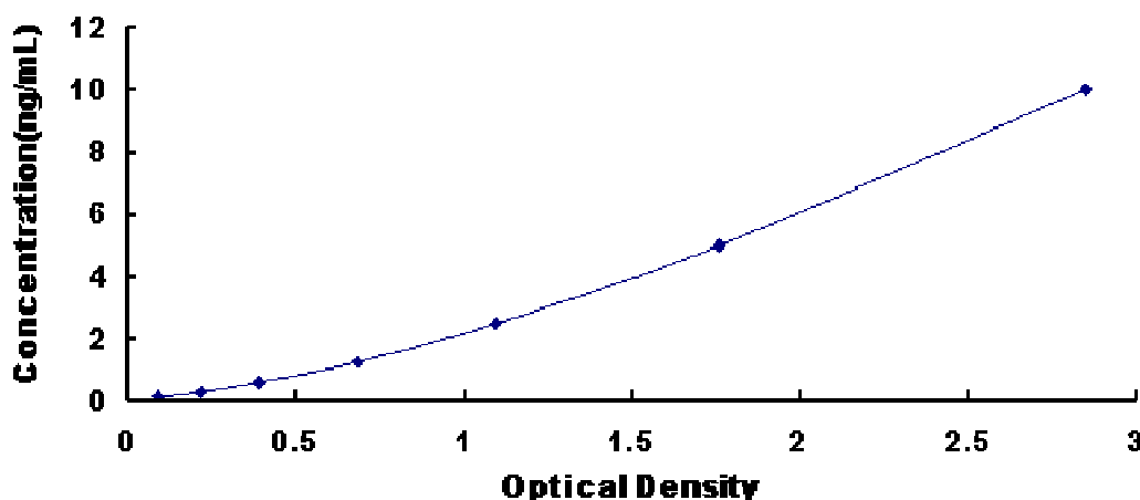
Typical Standard Curve for TLR7, Mouse ELISA.
