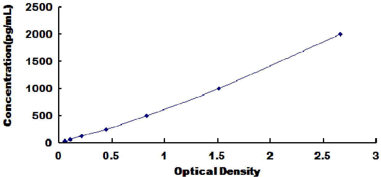
Typical Standard Curve for TIMP1, Porcine ELISA.
