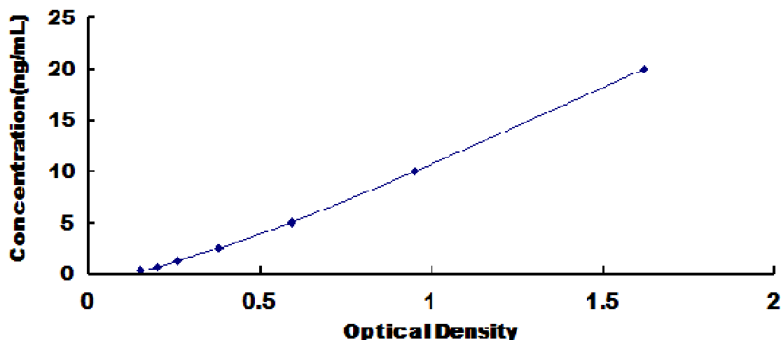
Typical Standard Curve for SPB, Rat ELISA.
