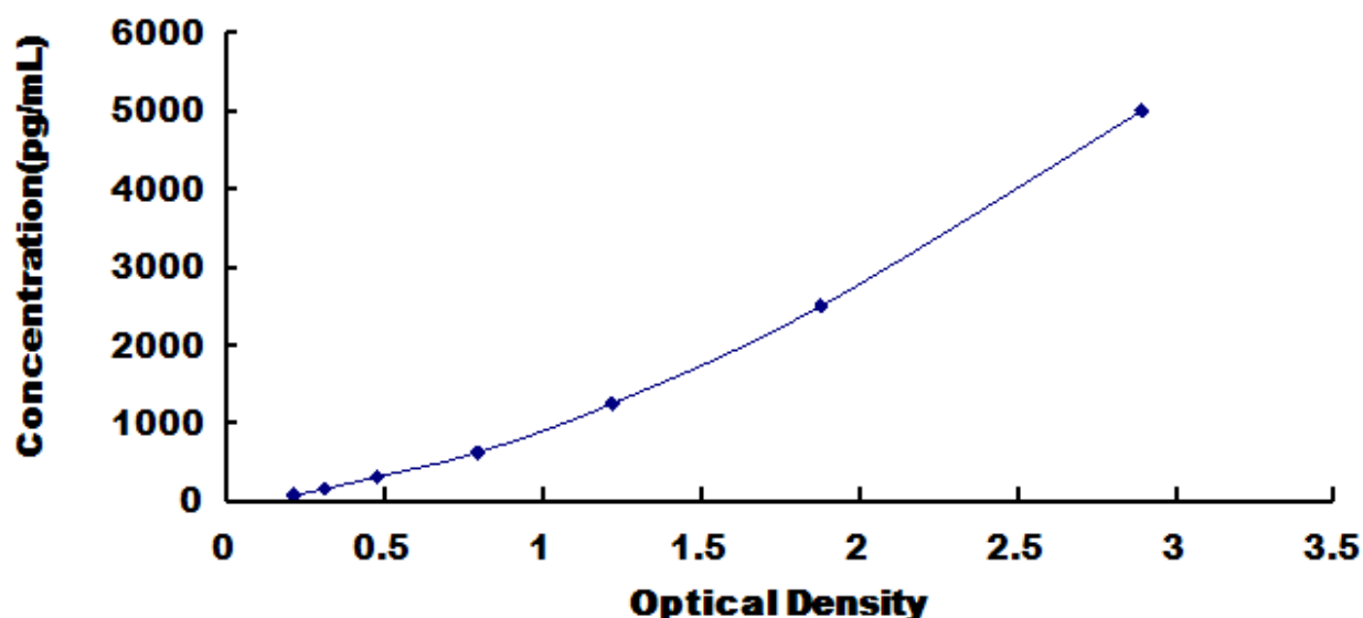
Typical Standard Curve for Slit2, Mouse ELISA.
