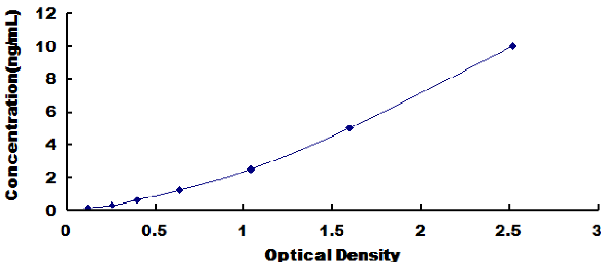
Typical Standard Curve for ARHGEF7, Rat ELISA.
