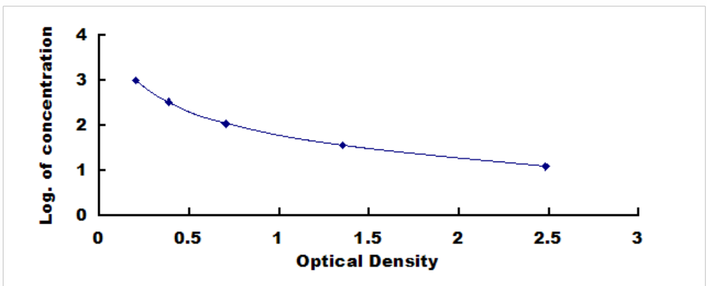
Typical Standard Curve for PGI 2 ELISA.
