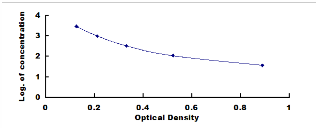
Typical Standard Curve for IGFIIE, Human ELISA.
