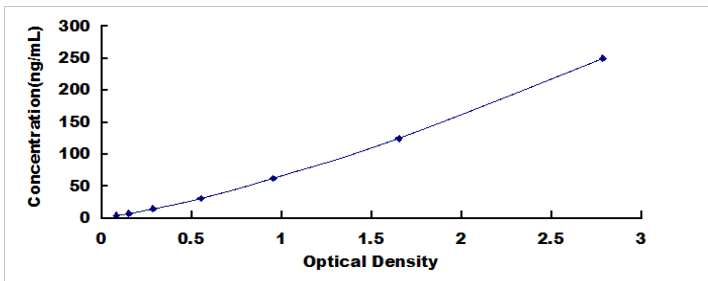
Typical Standard Curve for PLTP, Rat ELISA.
