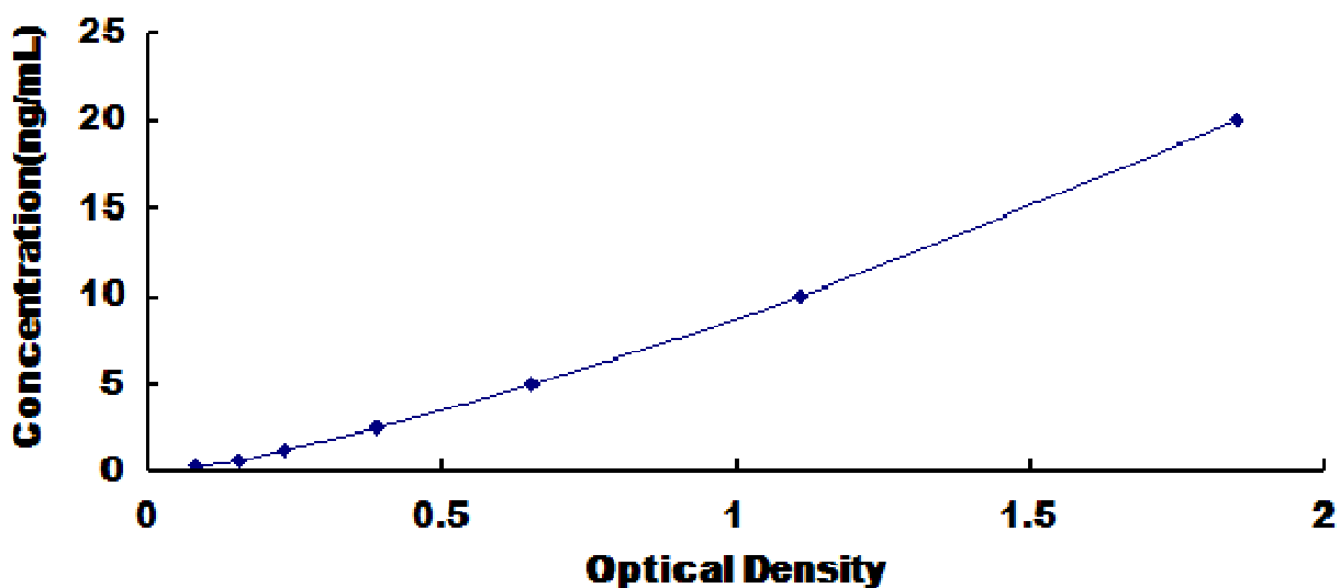
Typical Standard Curve for OSBPL8, Human ELISA.
