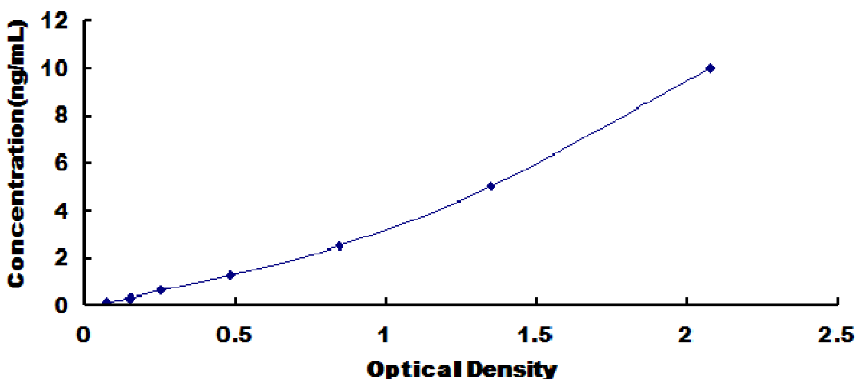
Typical Standard Curve for OSGIN1, Human ELISA.
