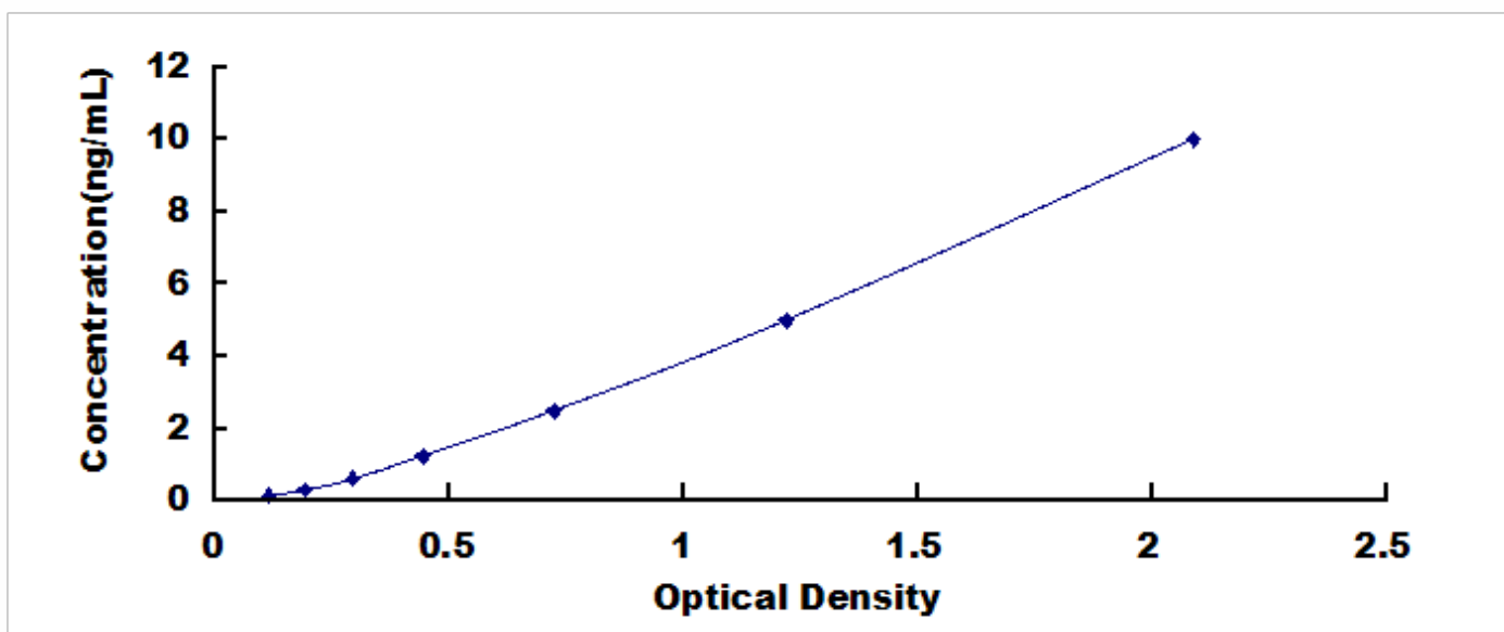
Typical Standard Curve for MyD88, Mouse ELISA.
