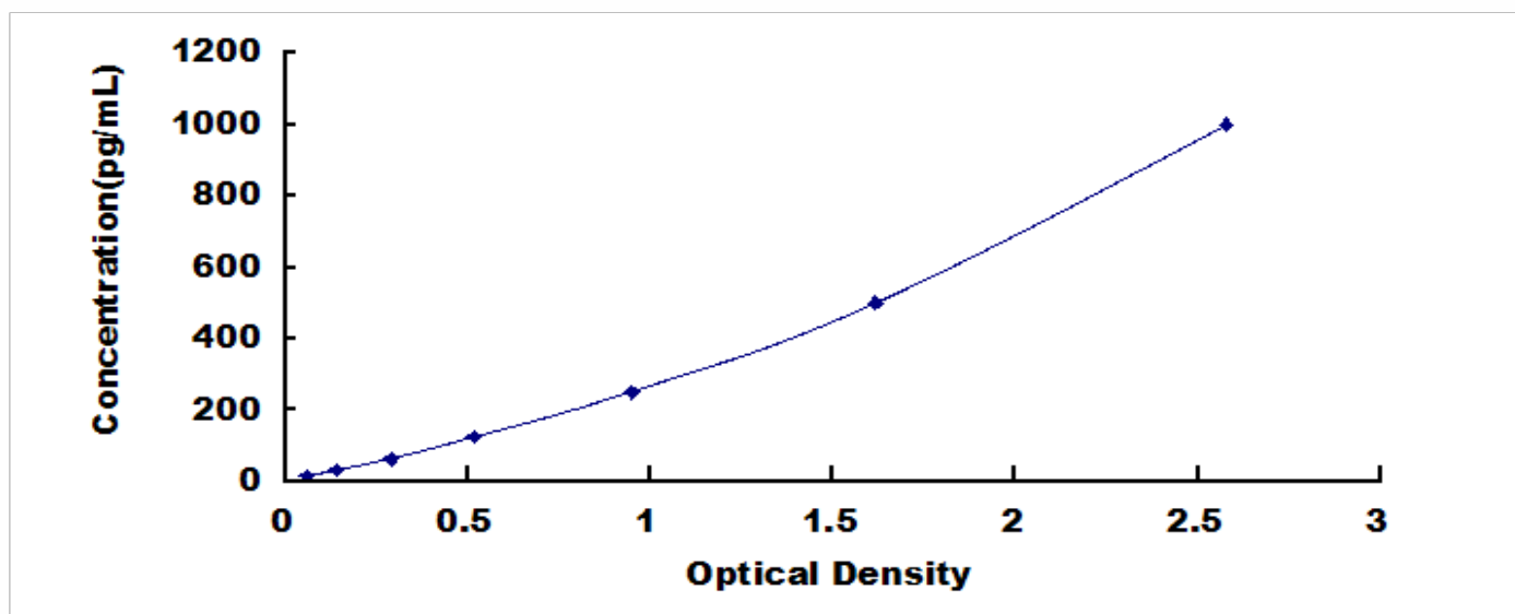
Typical Standard Curve for MBP, Mouse ELISA.
