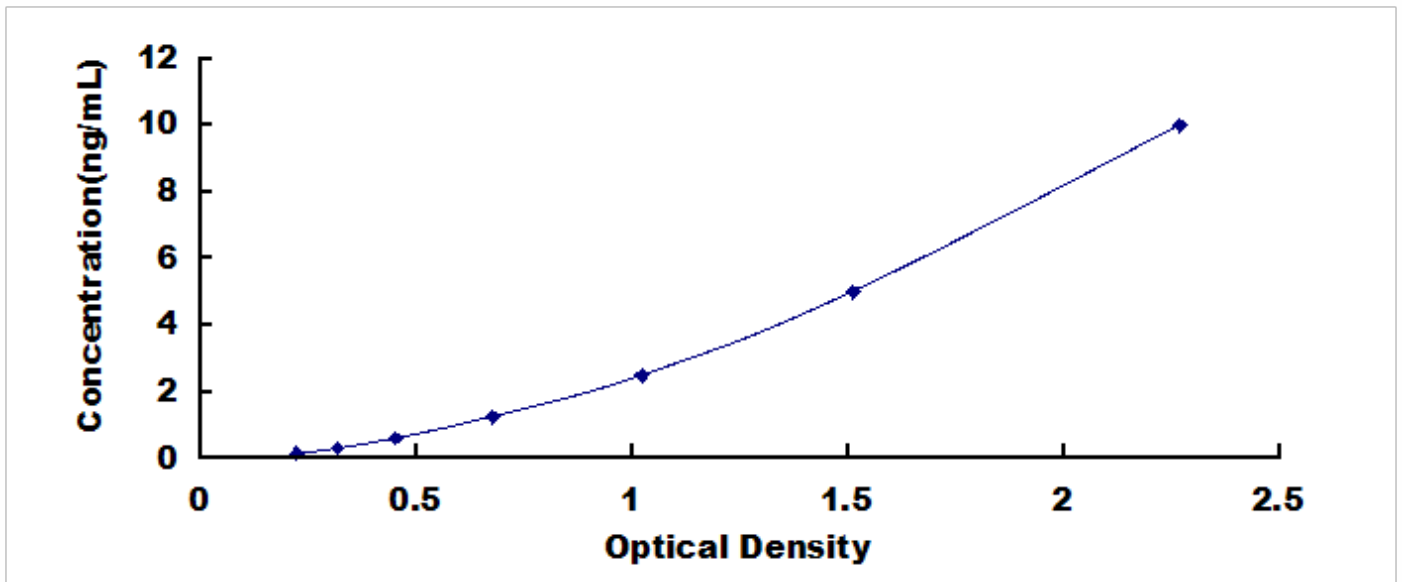
Typical Standard Curve for LFA1a, Mouse ELISA.
