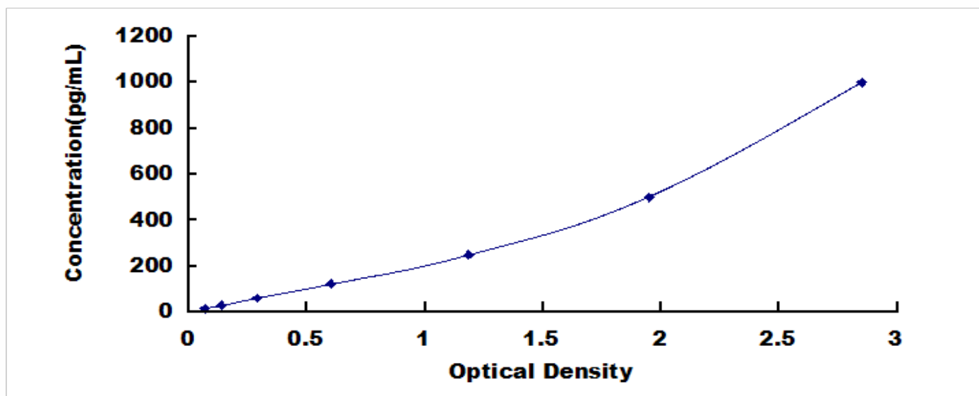
Typical Standard Curve for LAMC2, Human ELISA.
