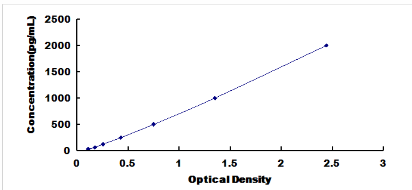
Typical Standard Curve for IL1RA, Bovine ELISA.
