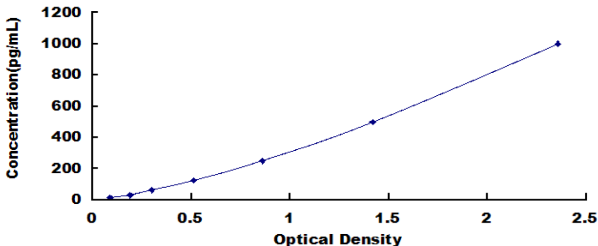
Typical Standard Curve for IL1a, Mouse ELISA.
