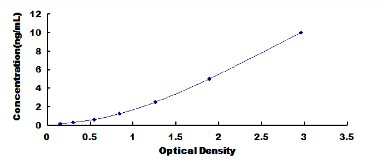
Typical Standard Curve for IRF3, Human ELISA.
