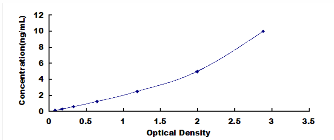
Typical Standard Curve for IGF1, Mouse ELISA.
