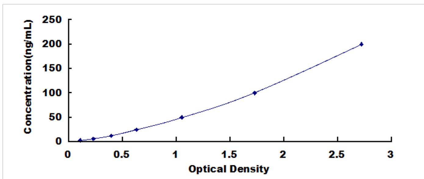
Typical Standard Curve for H2B ELISA.
