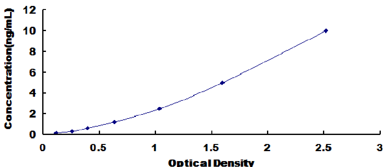
Typical Standard Curve for HO2, Human ELISA.
