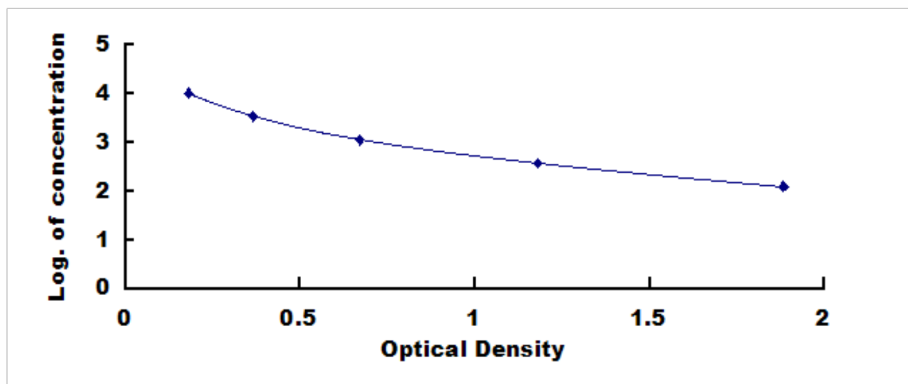
Typical Standard Curve for Ghrelin, Porcine ELISA.
