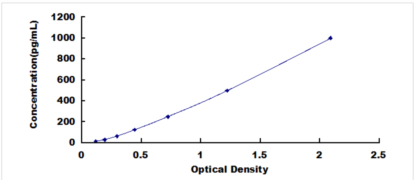
Typical Standard Curve for FCN2, Human ELISA.
