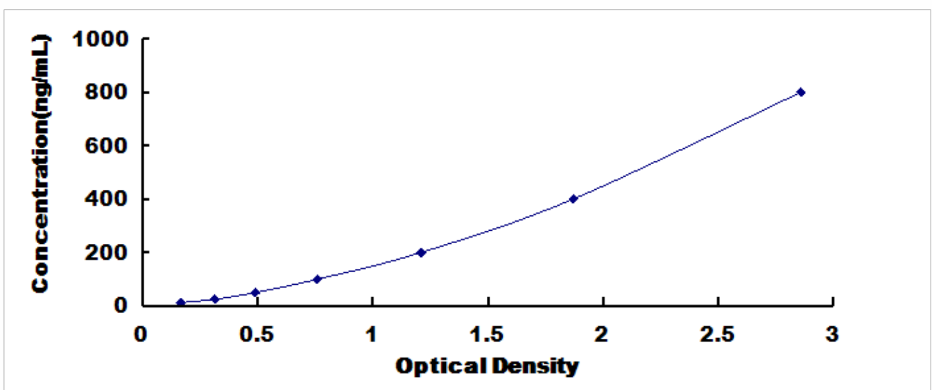
Typical Standard Curve for FG, Bovine ELISA.
