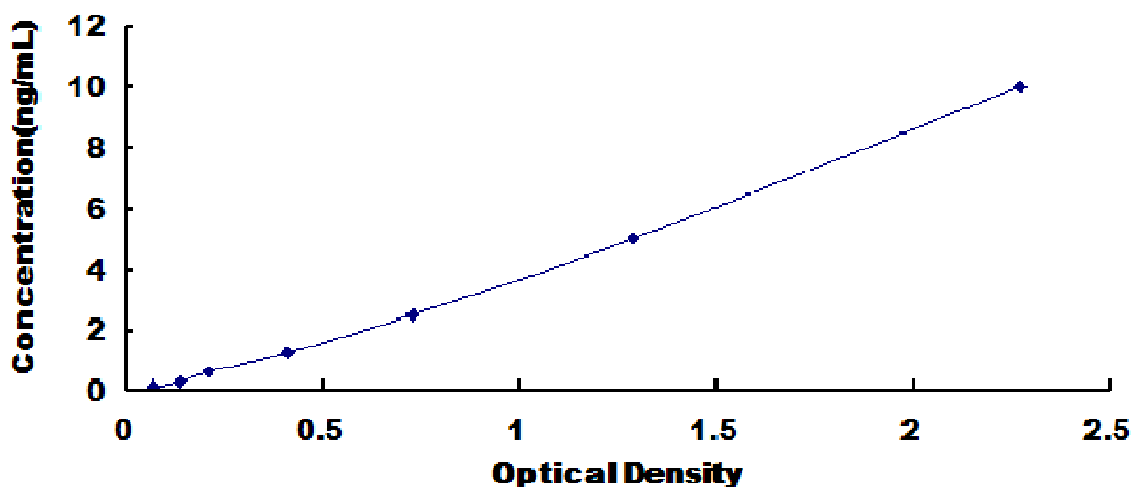
Typical Standard Curve for FTH, Mouse ELISA.
