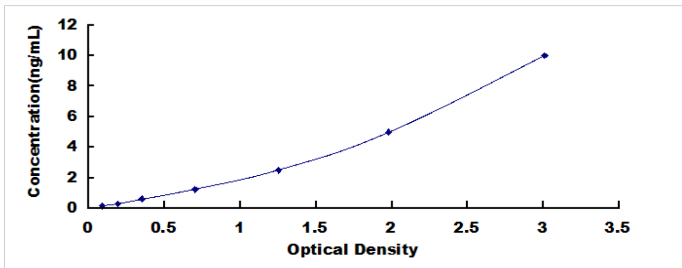
Typical Standard Curve for Ferritin, Human ELISA.
