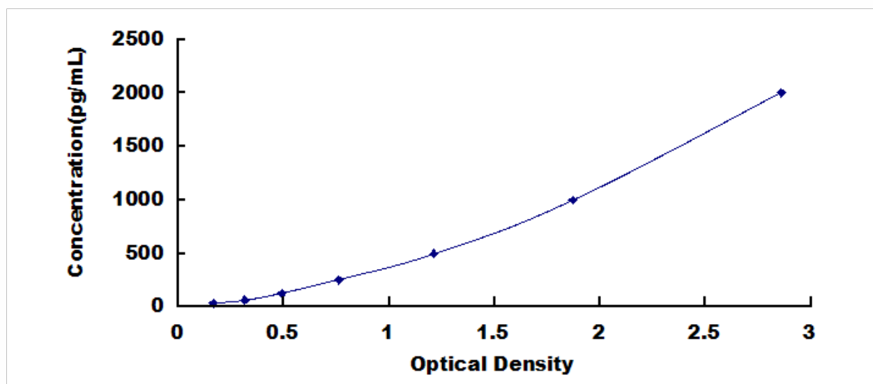
Typical Standard Curve for ENA78, Mouse ELISA.
