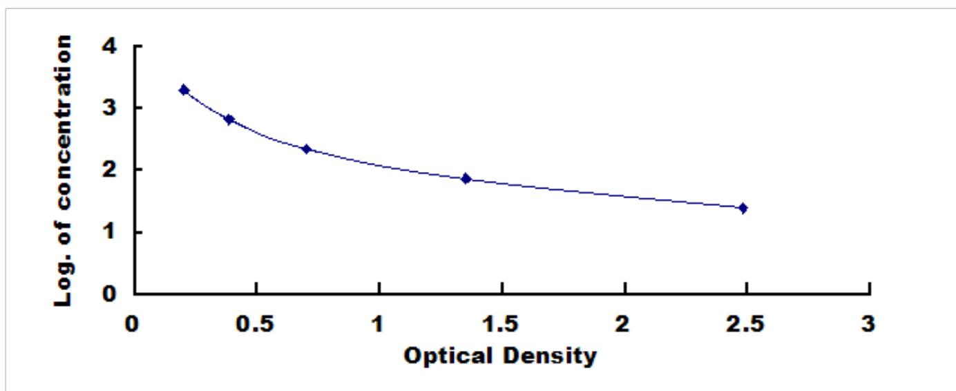
Typical Standard Curve for CPP, Mouse ELISA.
