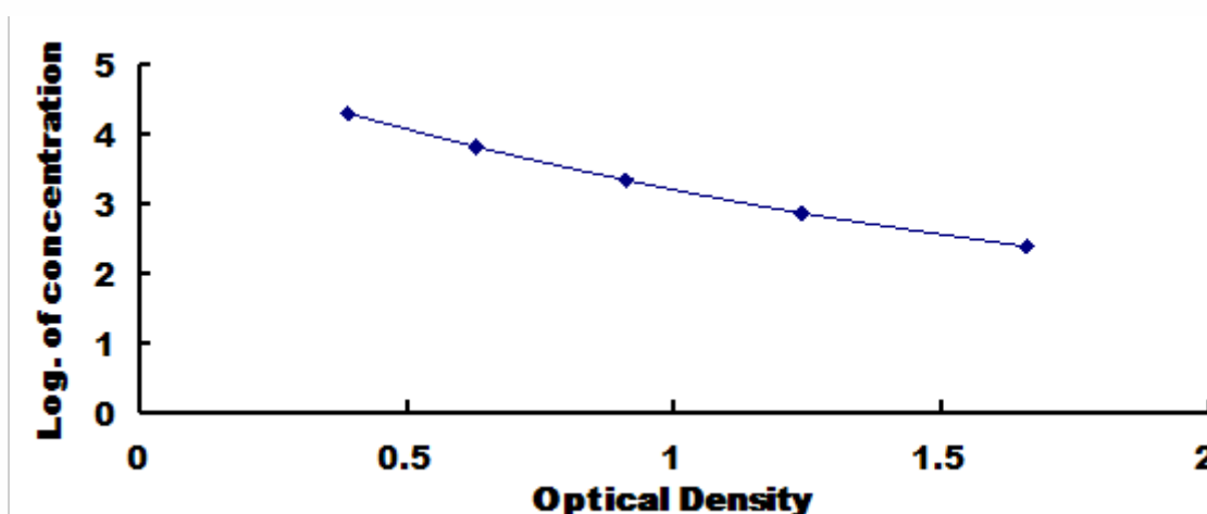
Typical Standard Curve for CPLX2, Human ELISA.
