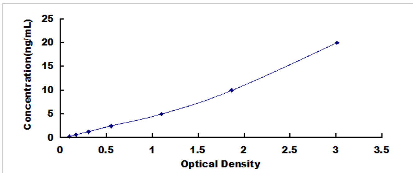
Typical Standard Curve for C4a, Rat ELISA.
