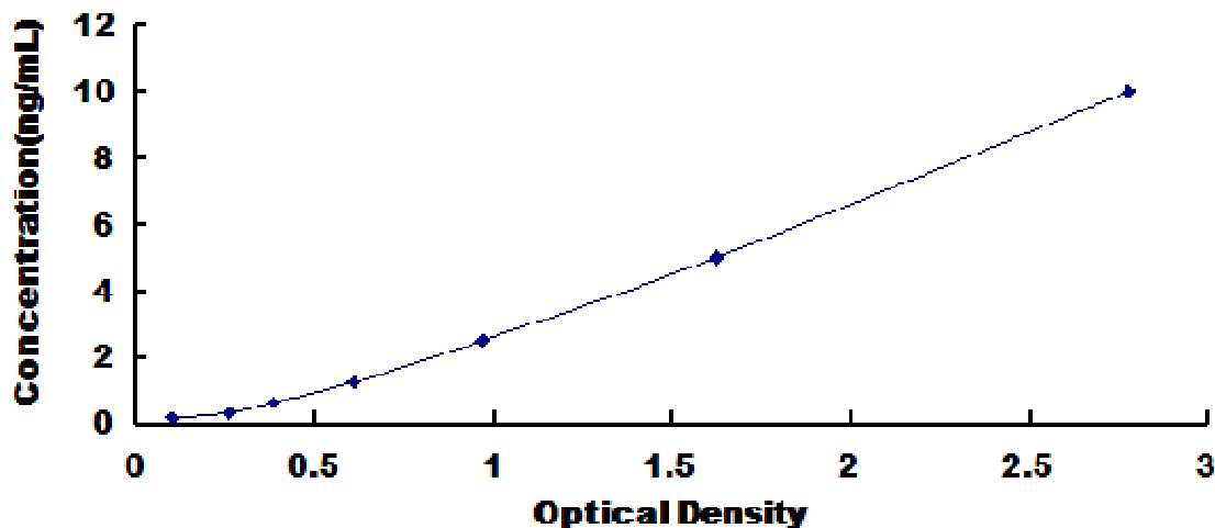
Typical Standard Curve for CDX2, Human ELISA.
