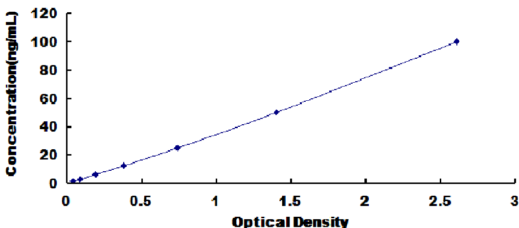
Typical Standard Curve for COMT, Rat ELISA.
