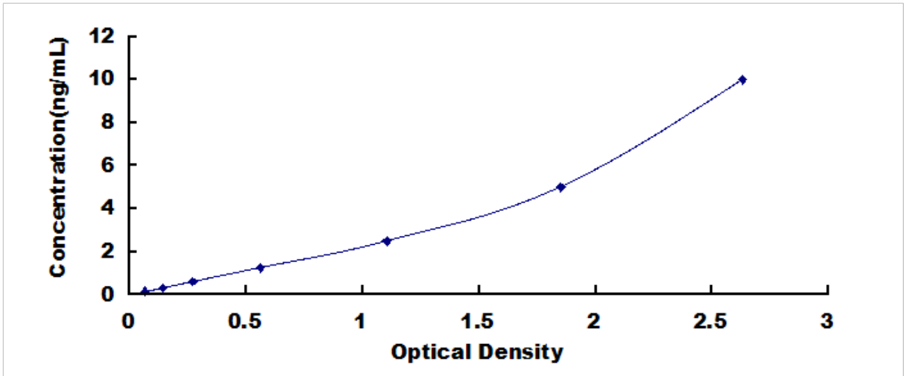
Typical Standard Curve for BDNF, Canine ELISA.
