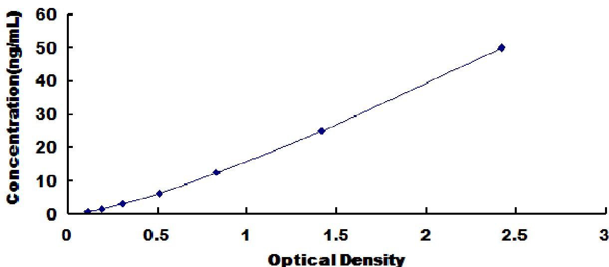
Typical Standard Curve for ASNS, Human ELISA.
