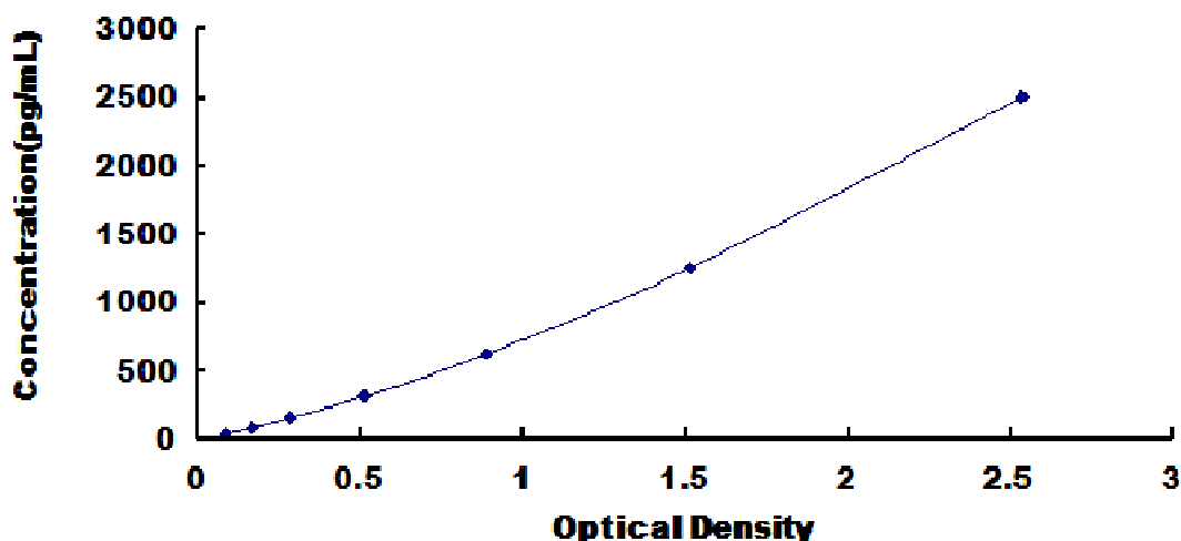
Typical Standard Curve for APOC2, Rat ELISA.
