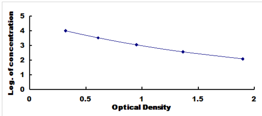
Typical Standard Curve for APOB100, Rabbit ELISA.
